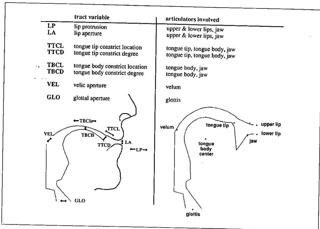
Fig. 1. Tract variables and associated articulators.
